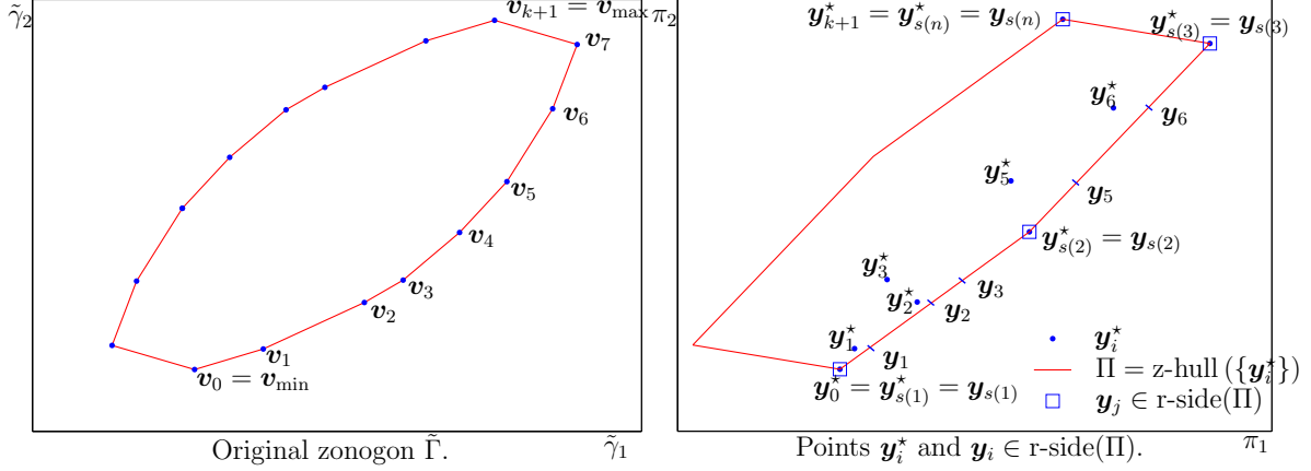
Figure 2-7: Matching and alignment performed in Algorithm 2.
