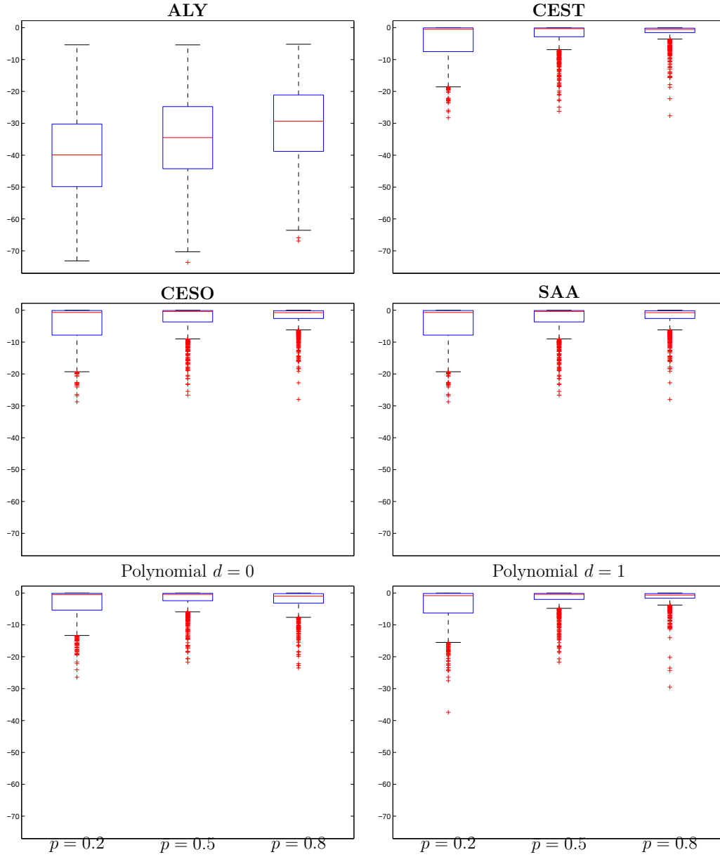
Figure C-7: Boxplots of relative gaps (in %) from perfect hindsight. Here, the coefficient \bar{p} varies, changing the mean of the perturbations. Testing distribution is the true one.
