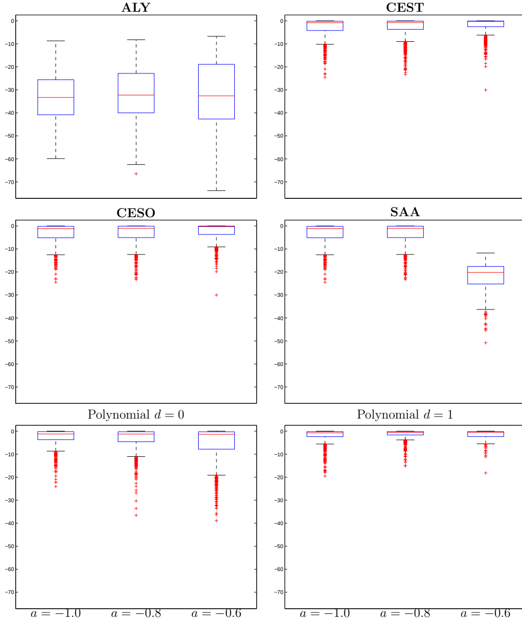
Figure C-5: Boxplots of relative gaps (in %) from perfect hindsight. Here, the noise terms u_t are Gaussian, and the value a in the price sensitivity matrix varies. Testing distribution is the true one.
