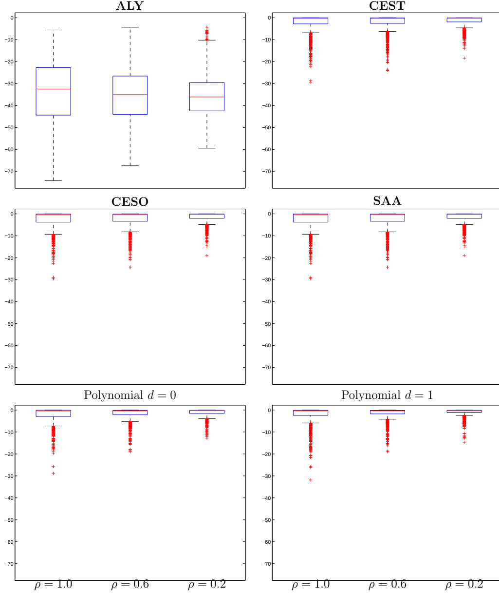
Figure C-3: Boxplots for the relative gaps (in %) from the perfect hindsight solution. Here, the noise terms u_t are Gaussian, and the correlation \rho varies, so as to make the disturbances in different time-periods less correlated. Testing distribution is the true one.
